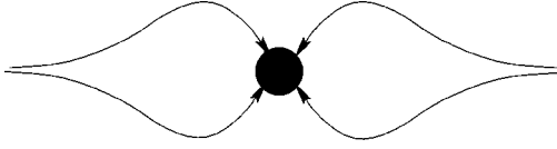
FIG. 3. A sketch of the field lines associated with the nexus-vortex combination of Eq. (33), gauge-transformed by the singular gauge transformation V . The Dirac strings are gone.
