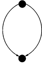
FIG. 1. Schematic picture of a nexus-vortex combination in SU(2) . A nexus and an anti-nexus are shown as black circles. They are joined by oppositely directed vortex segments.
