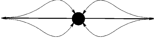
FIG. 2. A sketch of the field lines associated with the nexus-vortex combination of Eq. (25). The heavy straight lines are Dirac-string fields.
